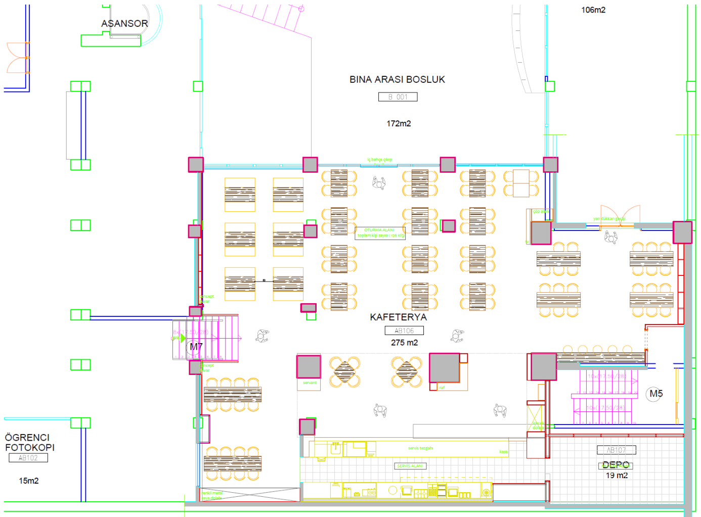
A BLOK 1.BODRUM KAT PLANI
