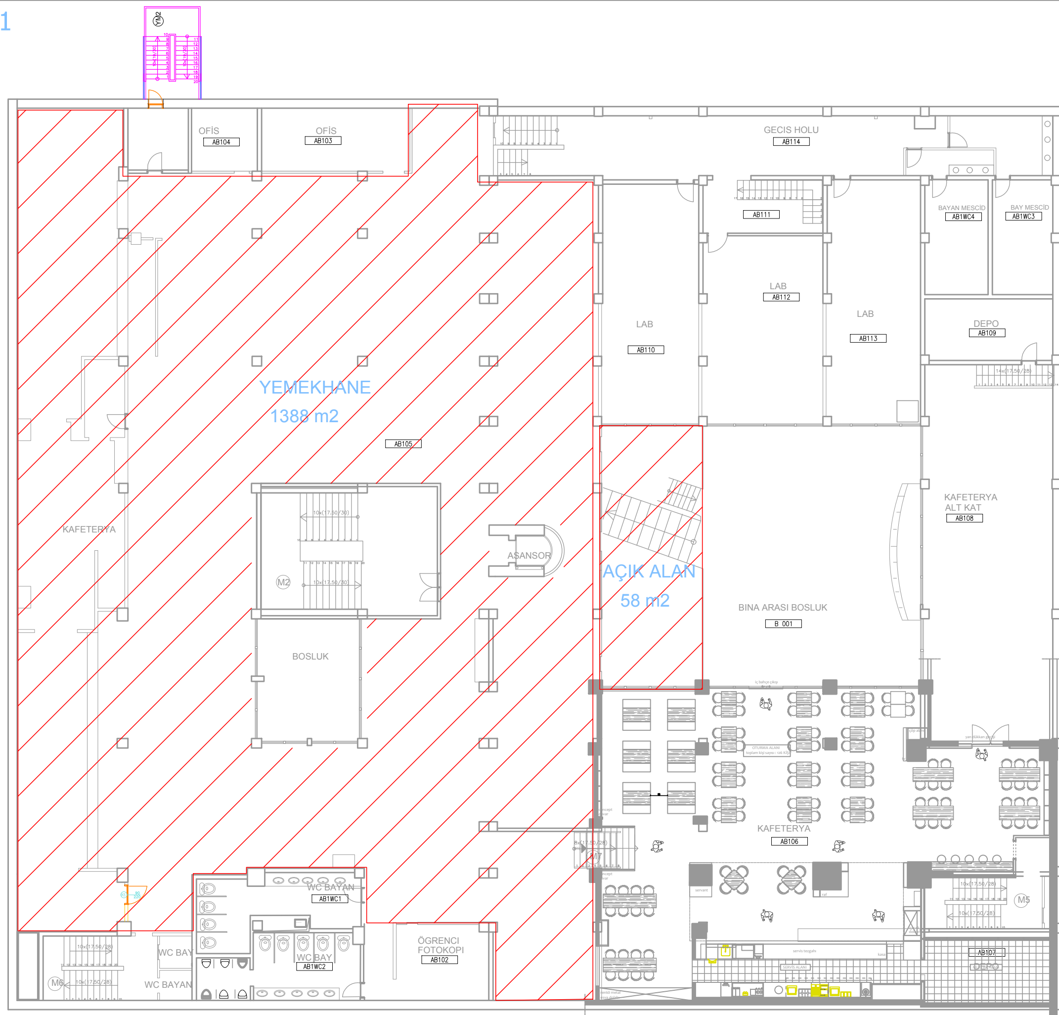
A BLOK 1.BODRUM KAT PLANI
